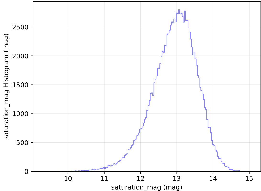
too_elab_r16_d2_ugrizy_v3.4_10yrs All sky u band: saturation_mag Histogram
