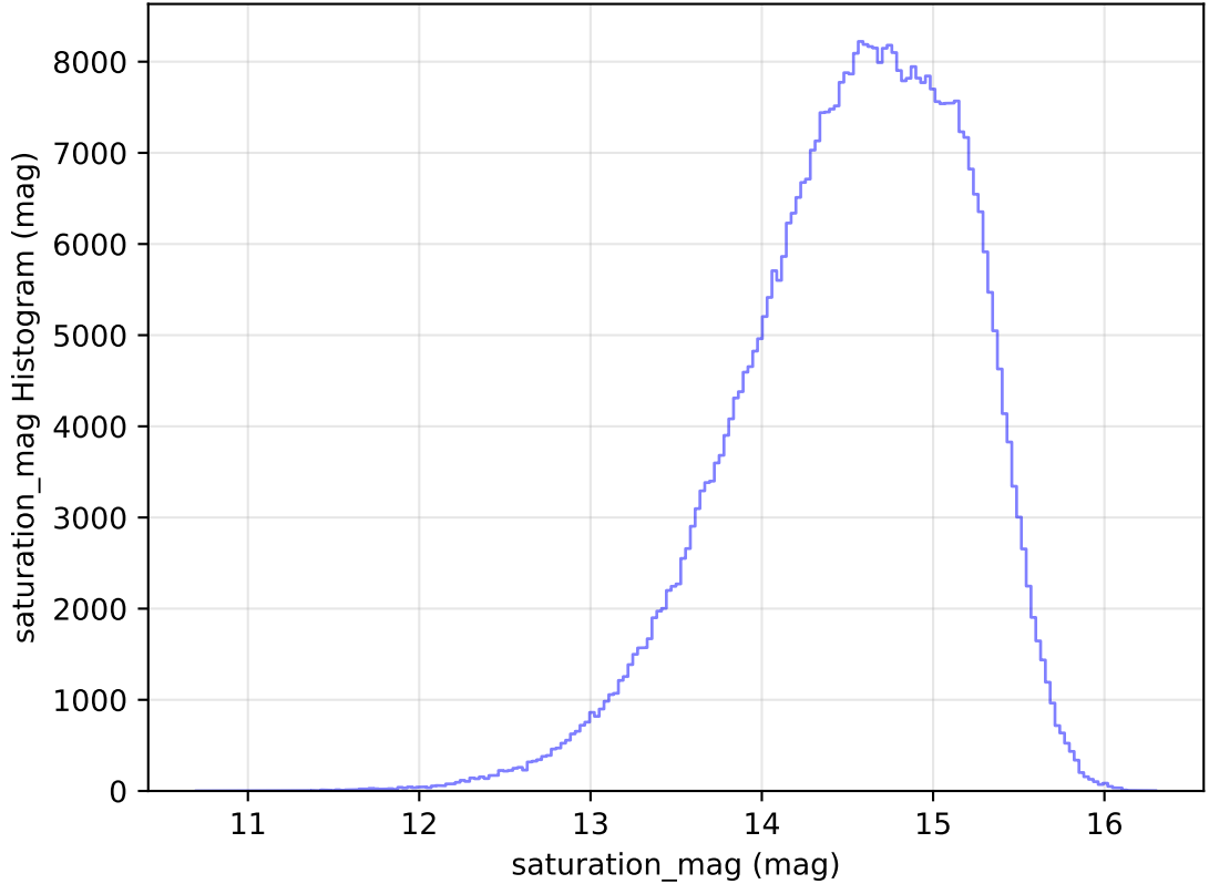
too_elab_r16_d2_ugrizy_v3.4_10yrs All sky r band: saturation_mag Histogram
