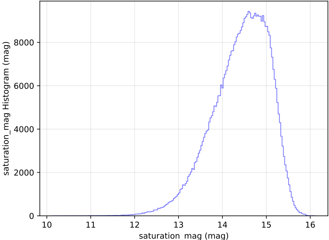
too_elab_r16_d2_ugrizy_v3.4_10yrs All sky i band: saturation_mag Histogram
