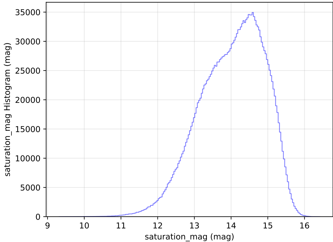
too_elab_r16_d2_ugrizy_v3.4_10yrs All sky all bands: saturation_mag Histogram
