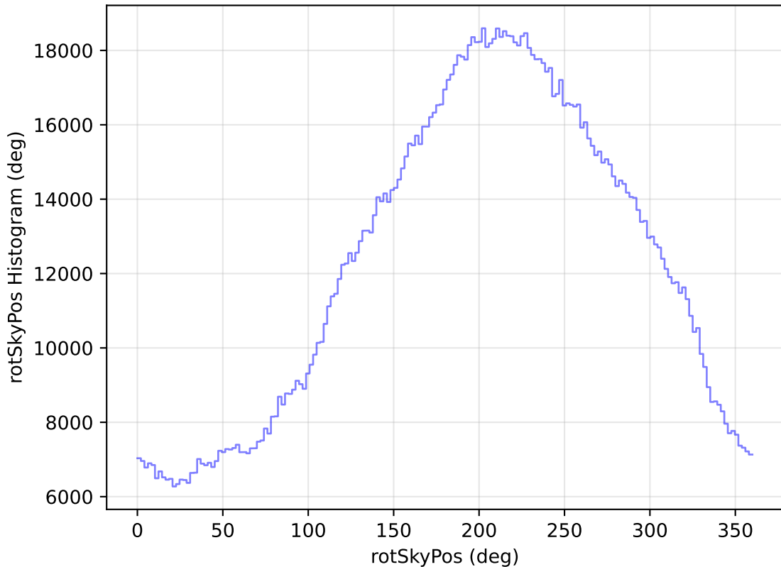
too_elab_r16_d2_ugrizy_v3.4_10yrs WFD all bands: rotSkyPos Histogram
