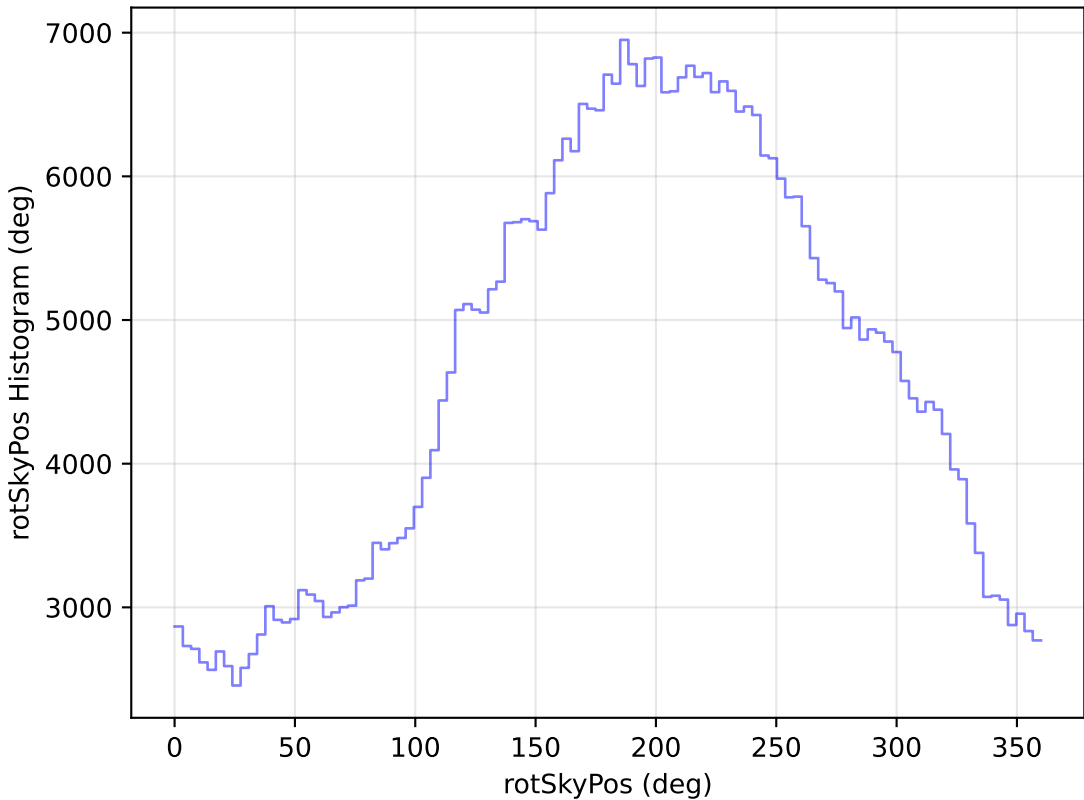
too_elab_r16_d2_ugrizy_v3.4_10yrs All sky r band: rotSkyPos Histogram
