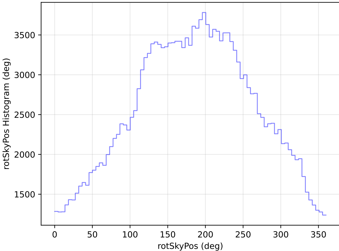
too_elab_r16_d2_ugrizy_v3.4_10yrs All sky g band: rotSkyPos Histogram
