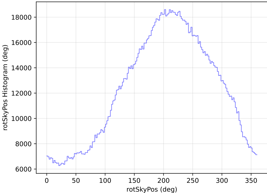
too_elab_r16_d2_ugrizy_v3.4_10yrs All sky all bands: rotSkyPos Histogram
