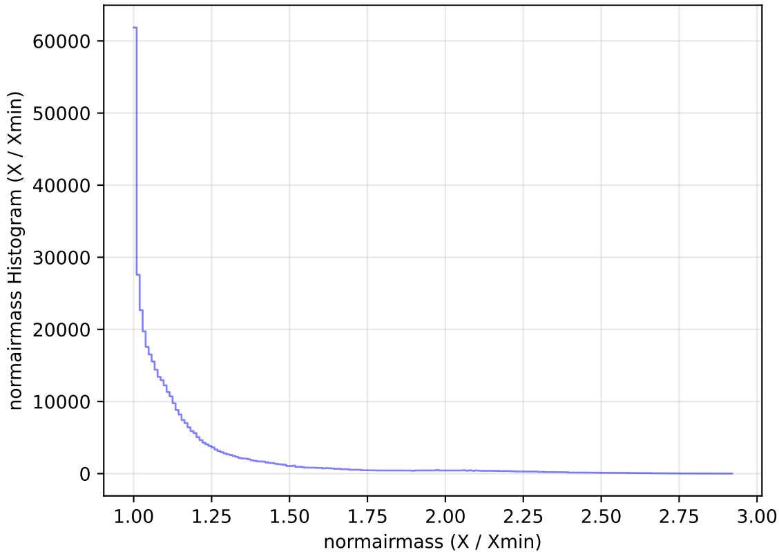
too_elab_r16_d2_ugrizy_v3.4_10yrs WFD z band: normairmass Histogram
