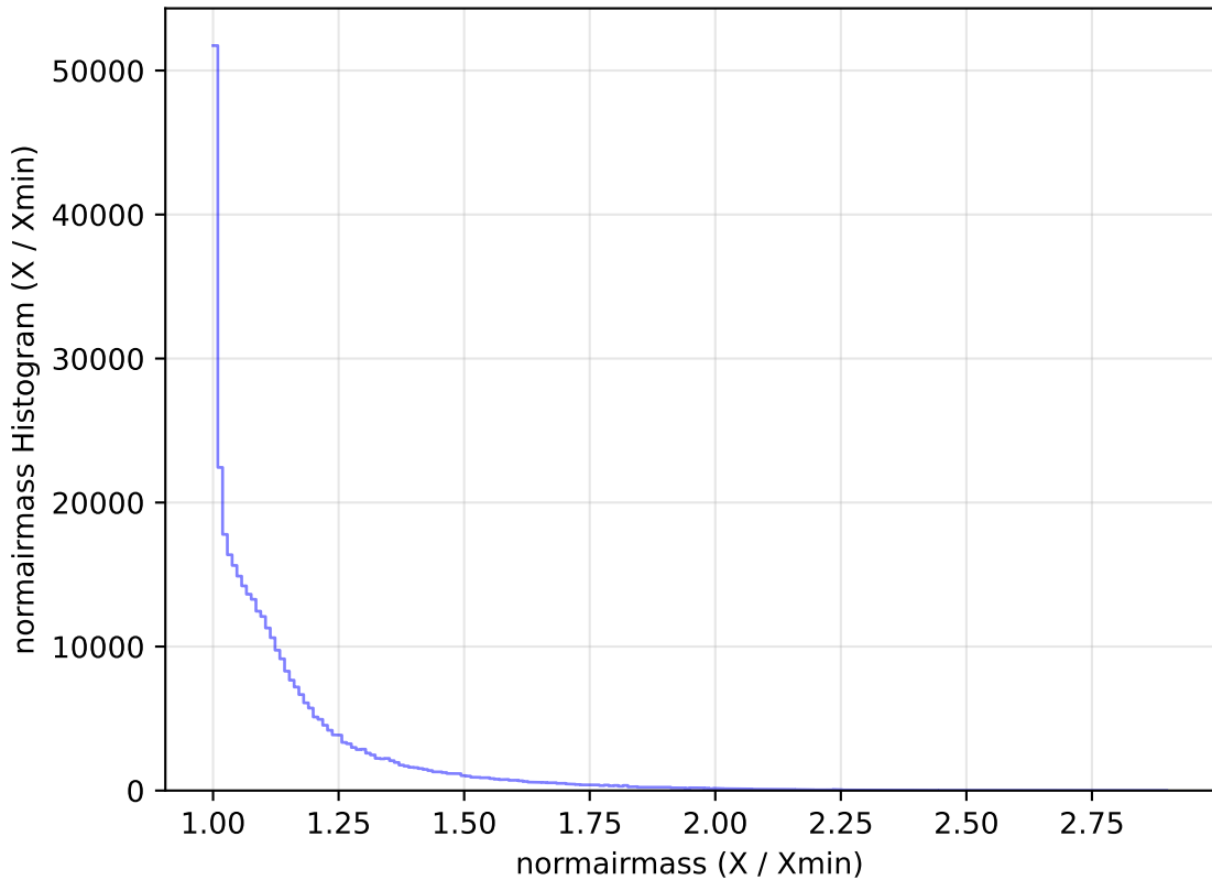
too_elab_r16_d2_ugrizy_v3.4_10yrs WFD y band: normairmass Histogram
