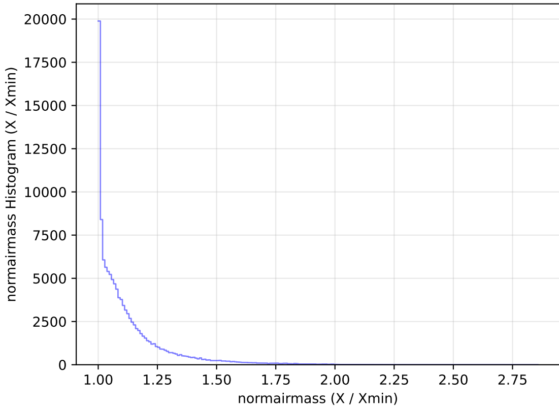
too_elab_r16_d2_ugrizy_v3.4_10yrs WFD u band: normairmass Histogram
