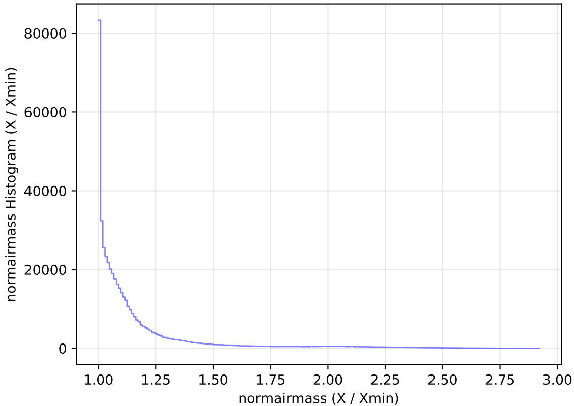
too_elab_r16_d2_ugrizy_v3.4_10yrs WFD i band: normairmass Histogram
