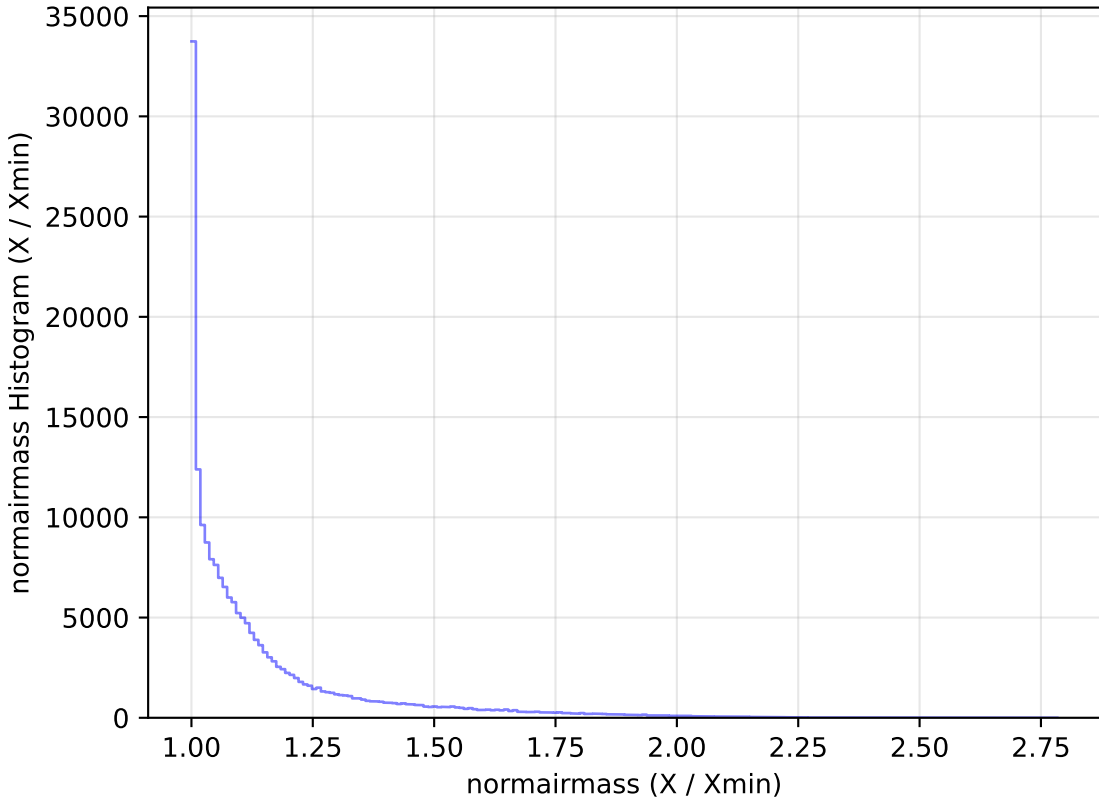
too_elab_r16_d2_ugrizy_v3.4_10yrs WFD g band: normairmass Histogram
