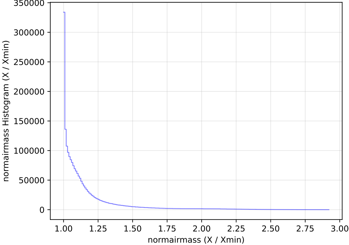
too_elab_r16_d2_ugrizy_v3.4_10yrs WFD all bands: normairmass Histogram
