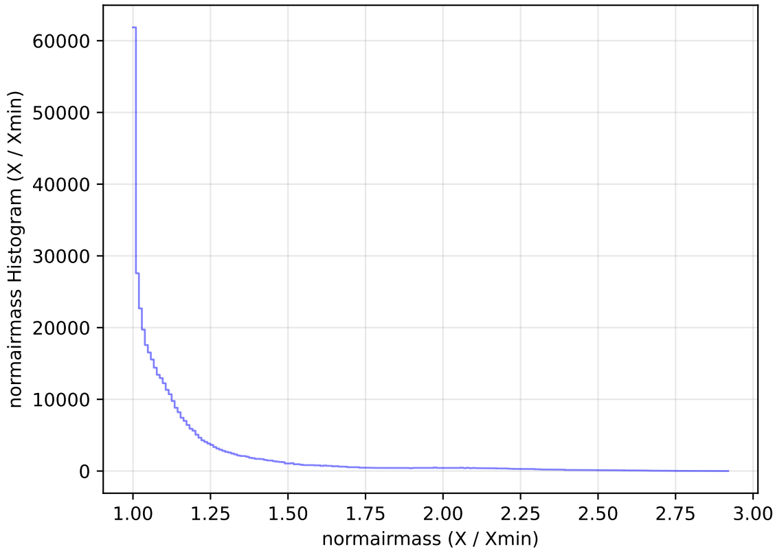
too_elab_r16_d2_ugrizy_v3.4_10yrs All sky z band: normairmass Histogram
