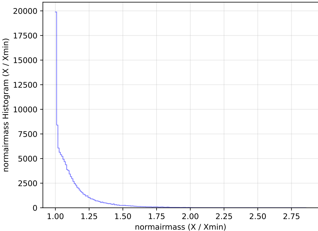
too_elab_r16_d2_ugrizy_v3.4_10yrs All sky u band: normairmass Histogram
