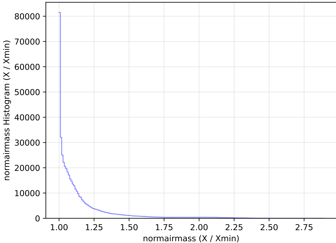
too_elab_r16_d2_ugrizy_v3.4_10yrs All sky r band: normairmass Histogram
