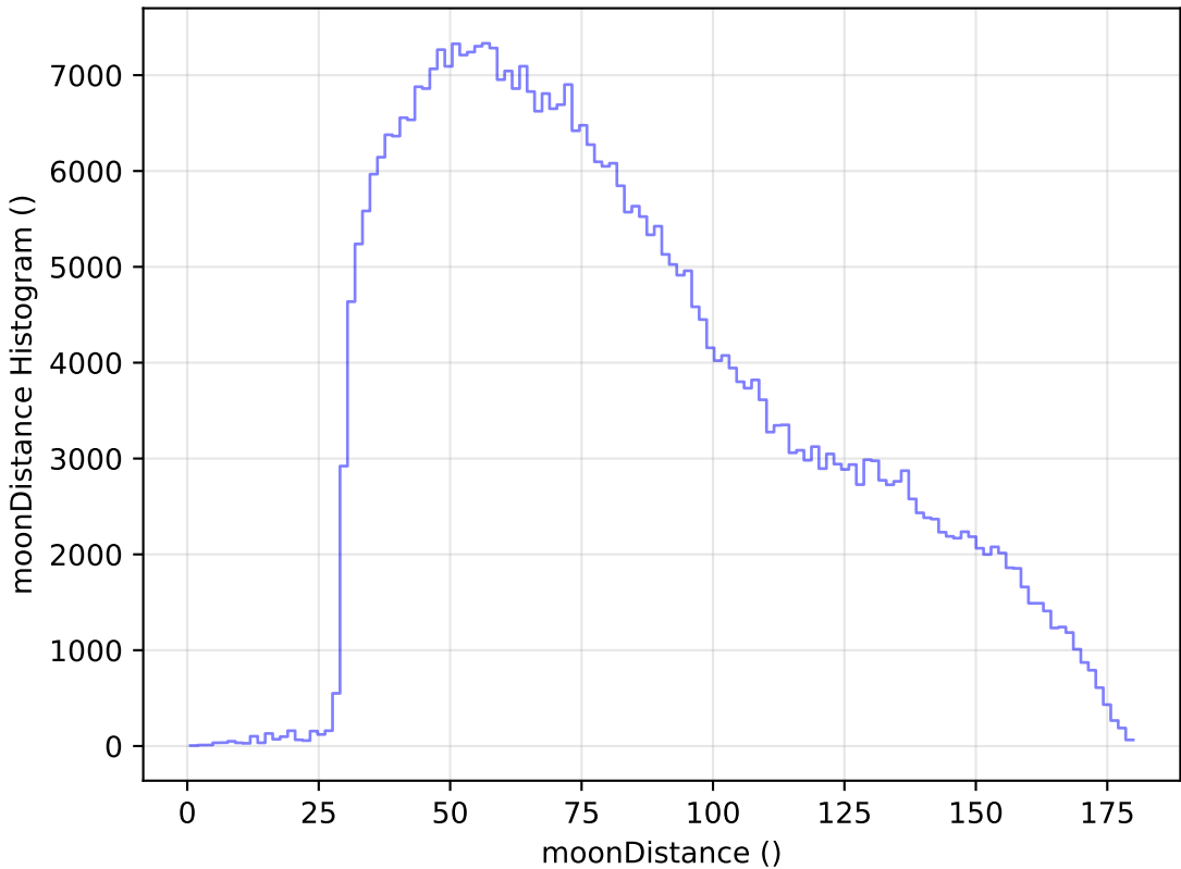
too_elab_r16_d2_ugrizy_v3.4_10yrs WFD z band: moonDistance Histogram
