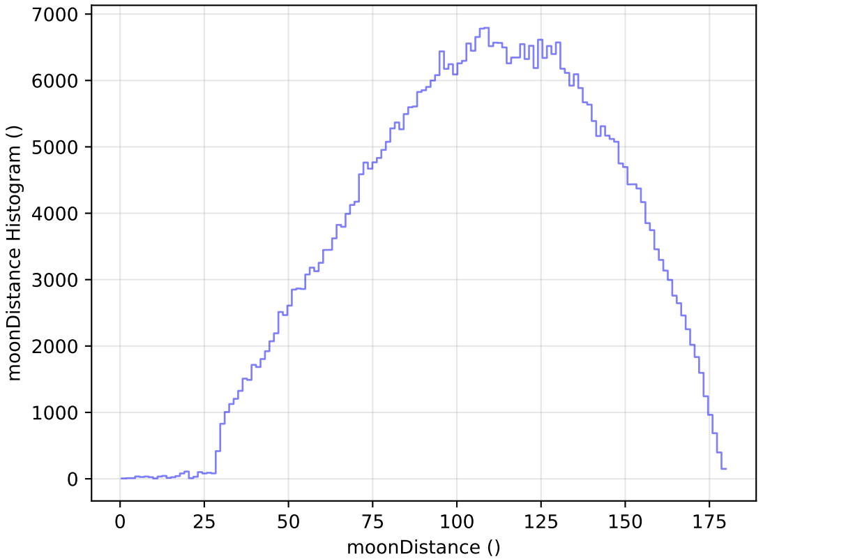
too_elab_r16_d2_ugrizy_v3.4_10yrs WFD r band: moonDistance Histogram
