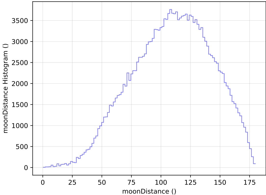
too_elab_r16_d2_ugrizy_v3.4_10yrs WFD g band: moonDistance Histogram
