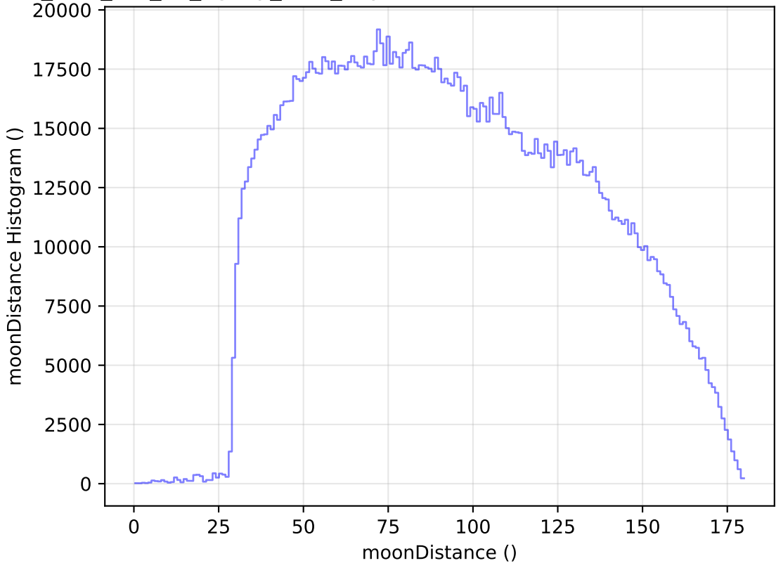
too_elab_r16_d2_ugrizy_v3.4_10yrs WFD all bands: moonDistance Histogram
