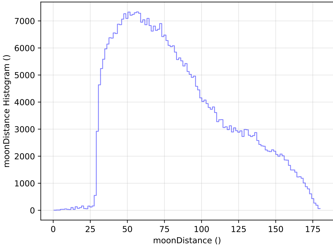
too_elab_r16_d2_ugrizy_v3.4_10yrs All sky z band: moonDistance Histogram
