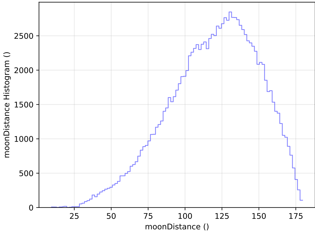
too_elab_r16_d2_ugrizy_v3.4_10yrs All sky u band: moonDistance Histogram
