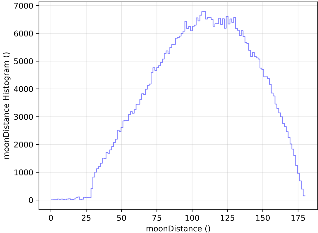
too_elab_r16_d2_ugrizy_v3.4_10yrs All sky r band: moonDistance Histogram
