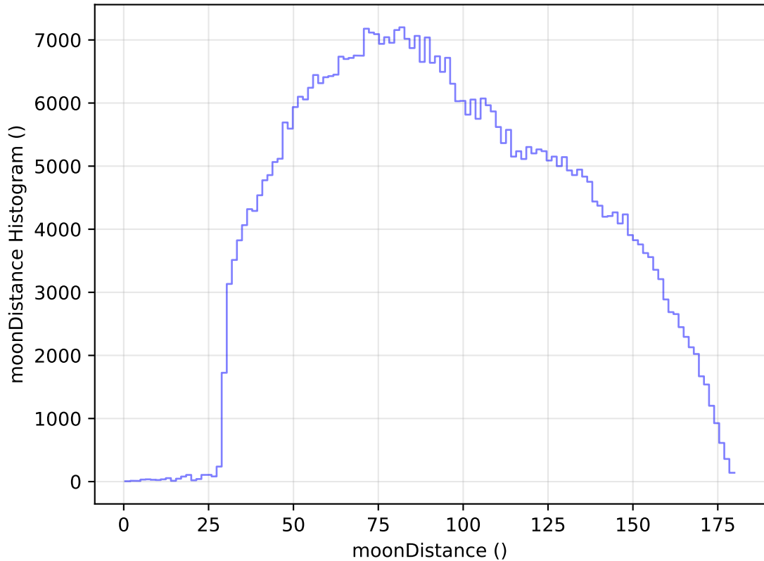
too_elab_r16_d2_ugrizy_v3.4_10yrs All sky i band: moonDistance Histogram
