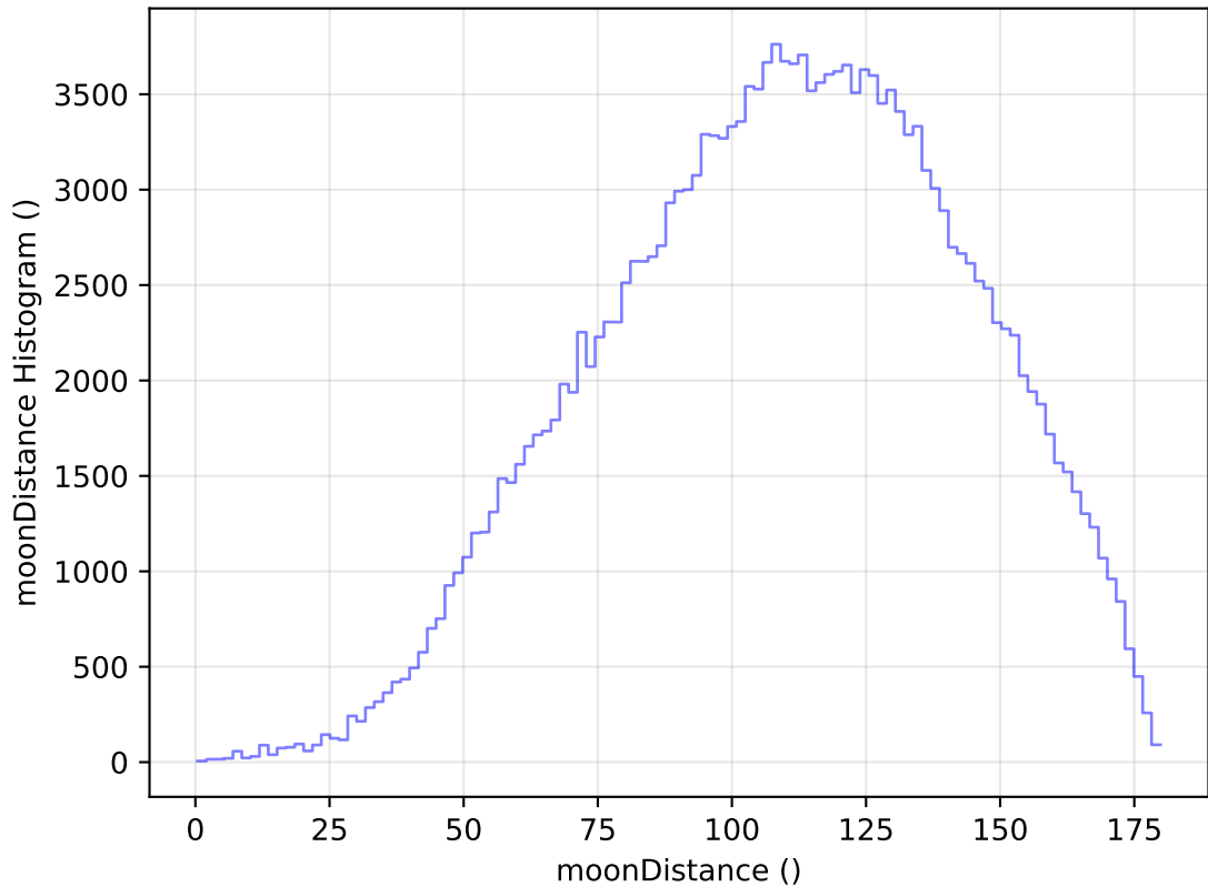
too_elab_r16_d2_ugrizy_v3.4_10yrs All sky g band: moonDistance Histogram
