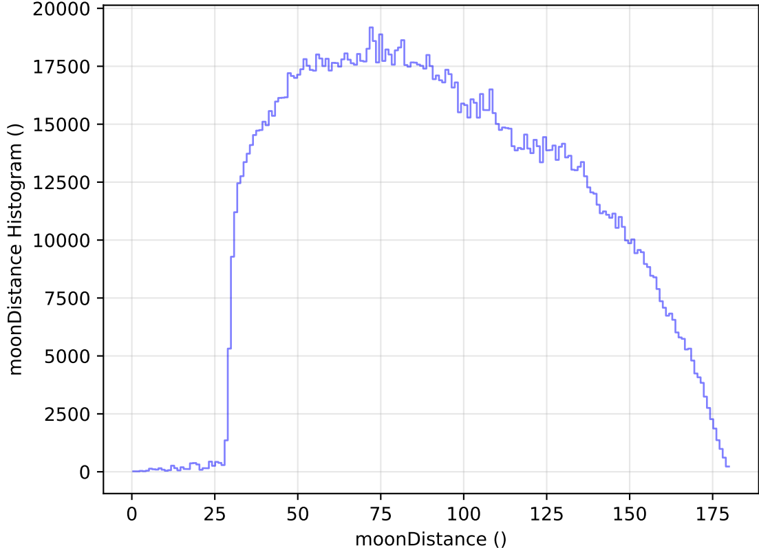
too_elab_r16_d2_ugrizy_v3.4_10yrs All sky all bands: moonDistance Histogram
