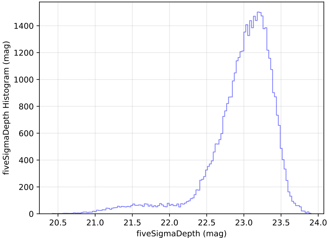
too_elab_r16_d2_ugrizy_v3.4_10yrs Yr 1 z band: fiveSigmaDepth Histogram
