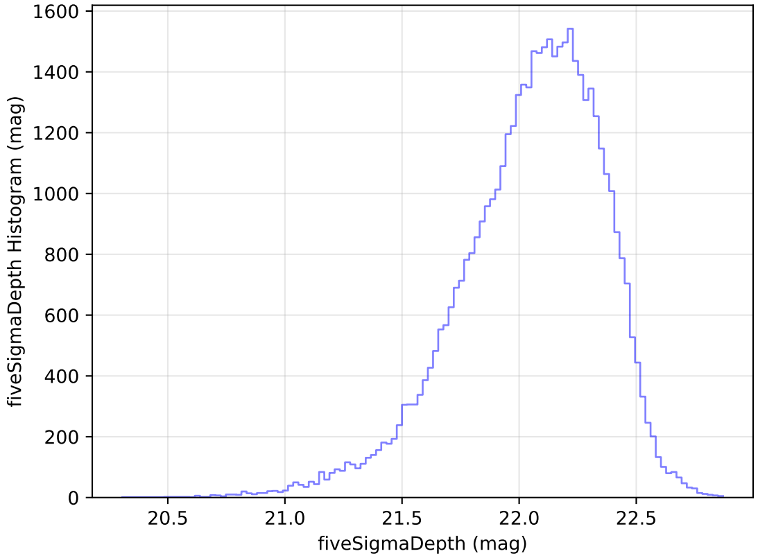
too_elab_r16_d2_ugrizy_v3.4_10yrs Yr 1 y band: fiveSigmaDepth Histogram
