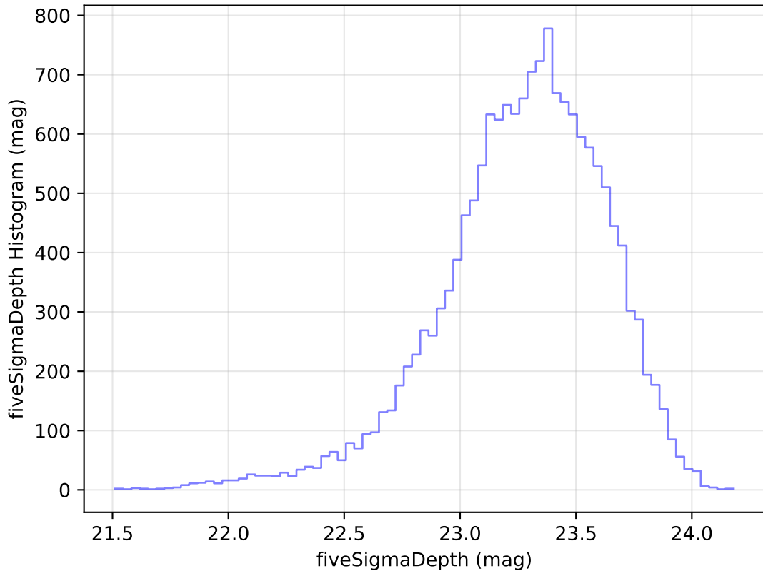
too_elab_r16_d2_ugrizy_v3.4_10yrs Yr 1 u band: fiveSigmaDepth Histogram
