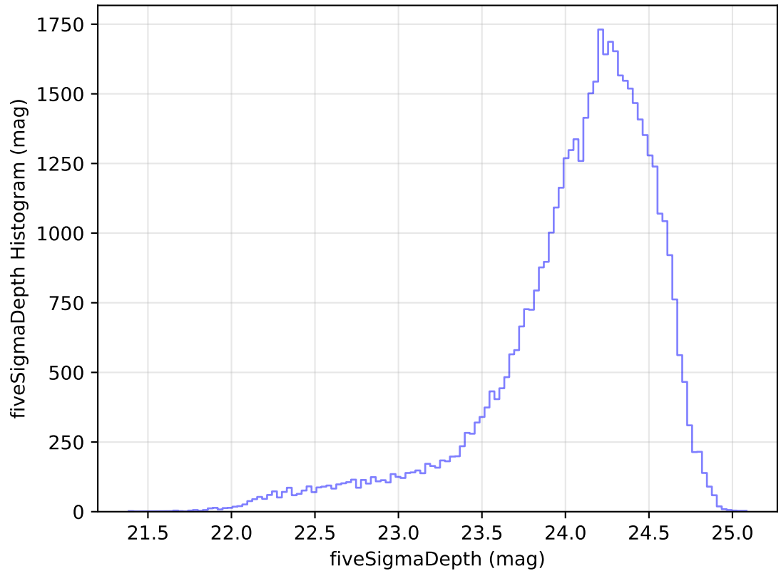
too_elab_r16_d2_ugrizy_v3.4_10yrs Yr 1 r band: fiveSigmaDepth Histogram
