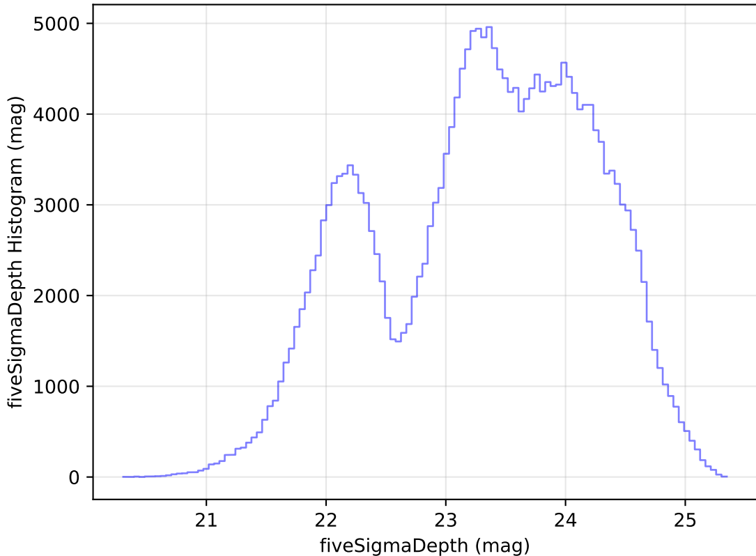
too_elab_r16_d2_ugrizy_v3.4_10yrs Yr 1 all bands: fiveSigmaDepth Histogram
