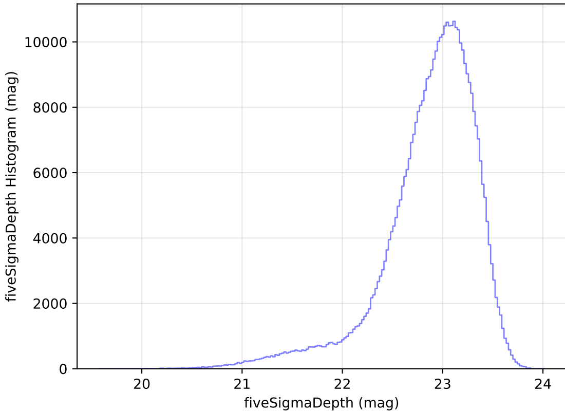
too_elab_r16_d2_ugrizy_v3.4_10yrs WFD z band: fiveSigmaDepth Histogram
