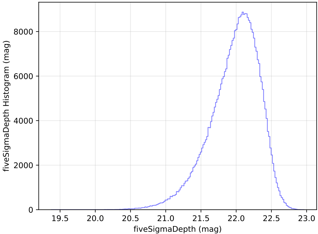
too_elab_r16_d2_ugrizy_v3.4_10yrs WFD y band: fiveSigmaDepth Histogram
