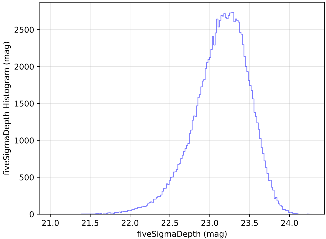
too_elab_r16_d2_ugrizy_v3.4_10yrs WFD u band: fiveSigmaDepth Histogram
