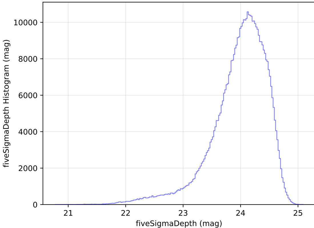
too_elab_r16_d2_ugrizy_v3.4_10yrs WFD r band: fiveSigmaDepth Histogram
