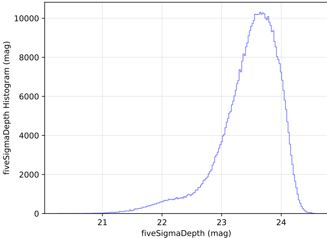
too_elab_r16_d2_ugrizy_v3.4_10yrs WFD i band: fiveSigmaDepth Histogram
