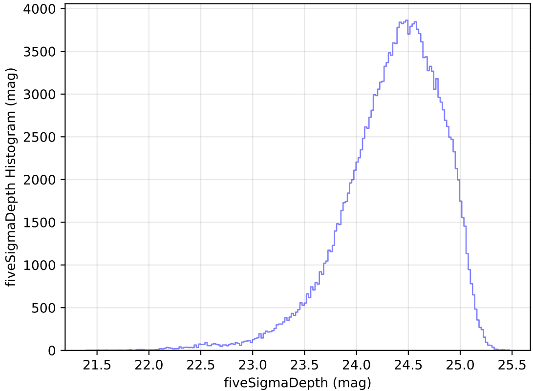
too_elab_r16_d2_ugrizy_v3.4_10yrs WFD g band: fiveSigmaDepth Histogram
