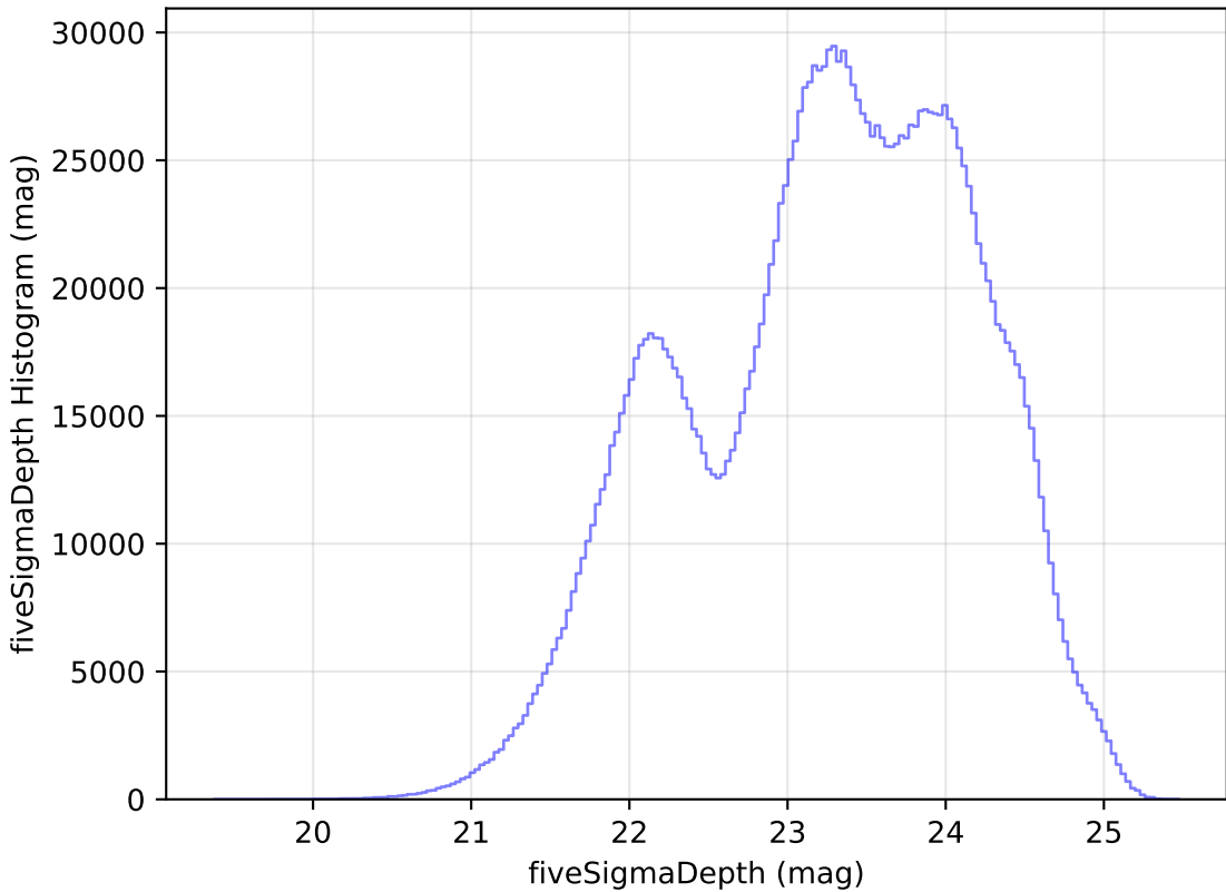
too_elab_r16_d2_ugrizy_v3.4_10yrs WFD all bands: fiveSigmaDepth Histogram
