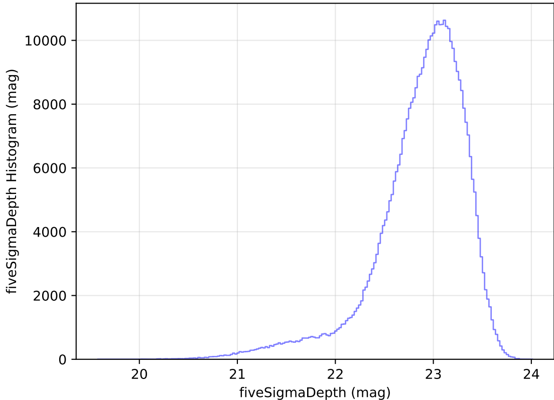
too_elab_r16_d2_ugrizy_v3.4_10yrs All sky z band: fiveSigmaDepth Histogram
