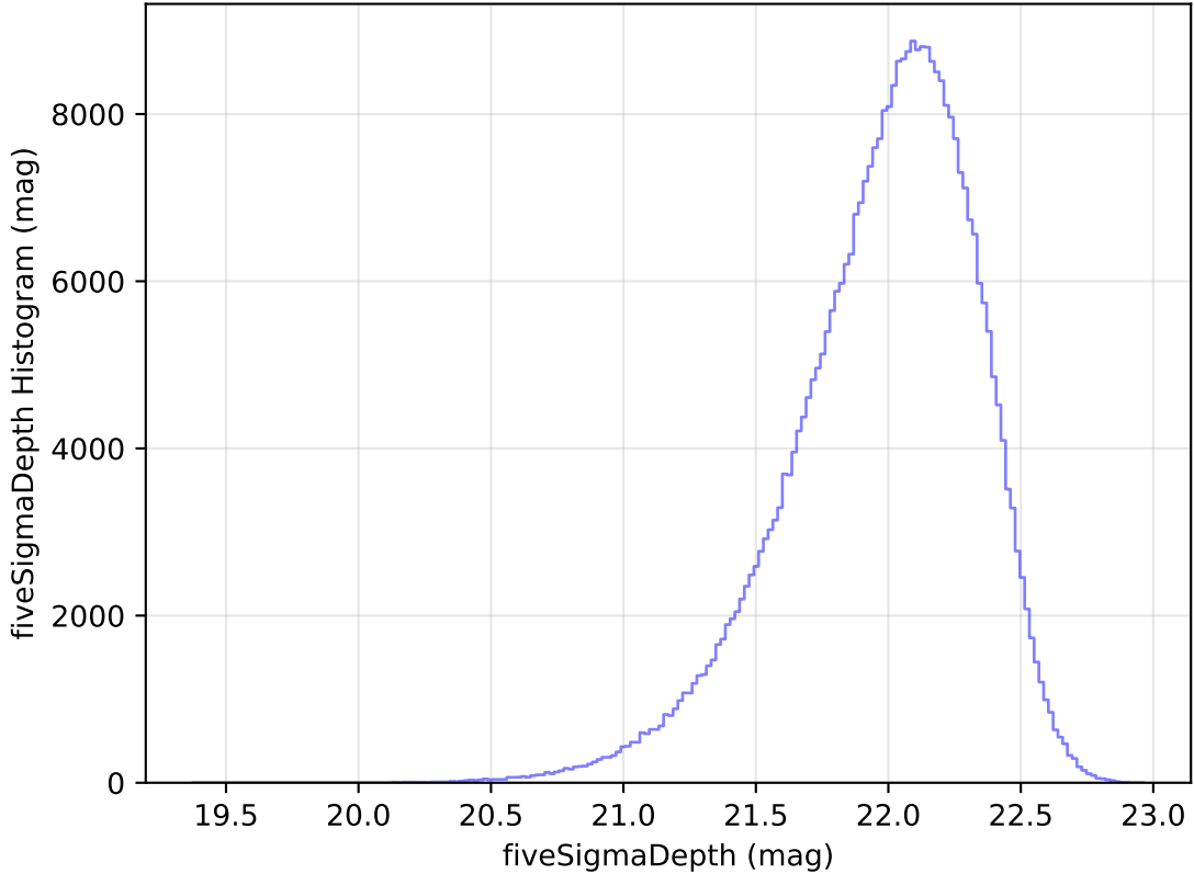
too_elab_r16_d2_ugrizy_v3.4_10yrs All sky y band: fiveSigmaDepth Histogram
