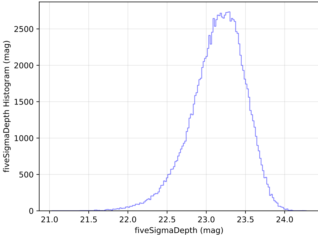
too_elab_r16_d2_ugrizy_v3.4_10yrs All sky u band: fiveSigmaDepth Histogram
