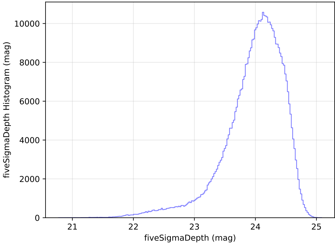
too_elab_r16_d2_ugrizy_v3.4_10yrs All sky r band: fiveSigmaDepth Histogram
