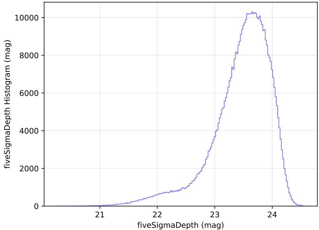
too_elab_r16_d2_ugrizy_v3.4_10yrs All sky i band: fiveSigmaDepth Histogram
