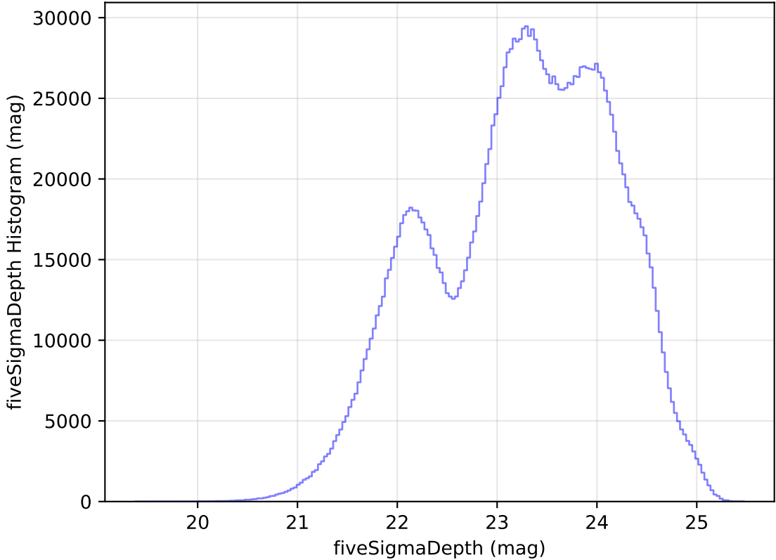
too_elab_r16_d2_ugrizy_v3.4_10yrs All sky all bands: fiveSigmaDepth Histogram
