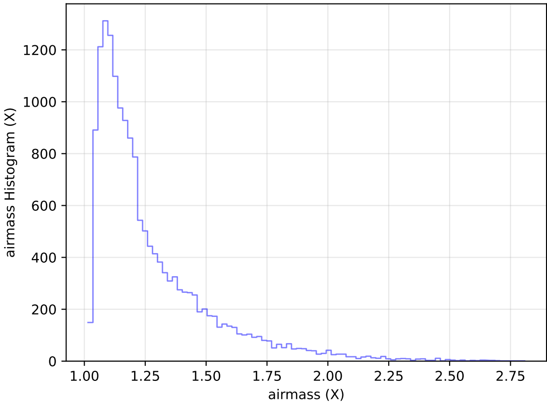
too_elab_r16_d2_ugrizy_v3.4_10yrs Yr 1 u band: airmass Histogram
