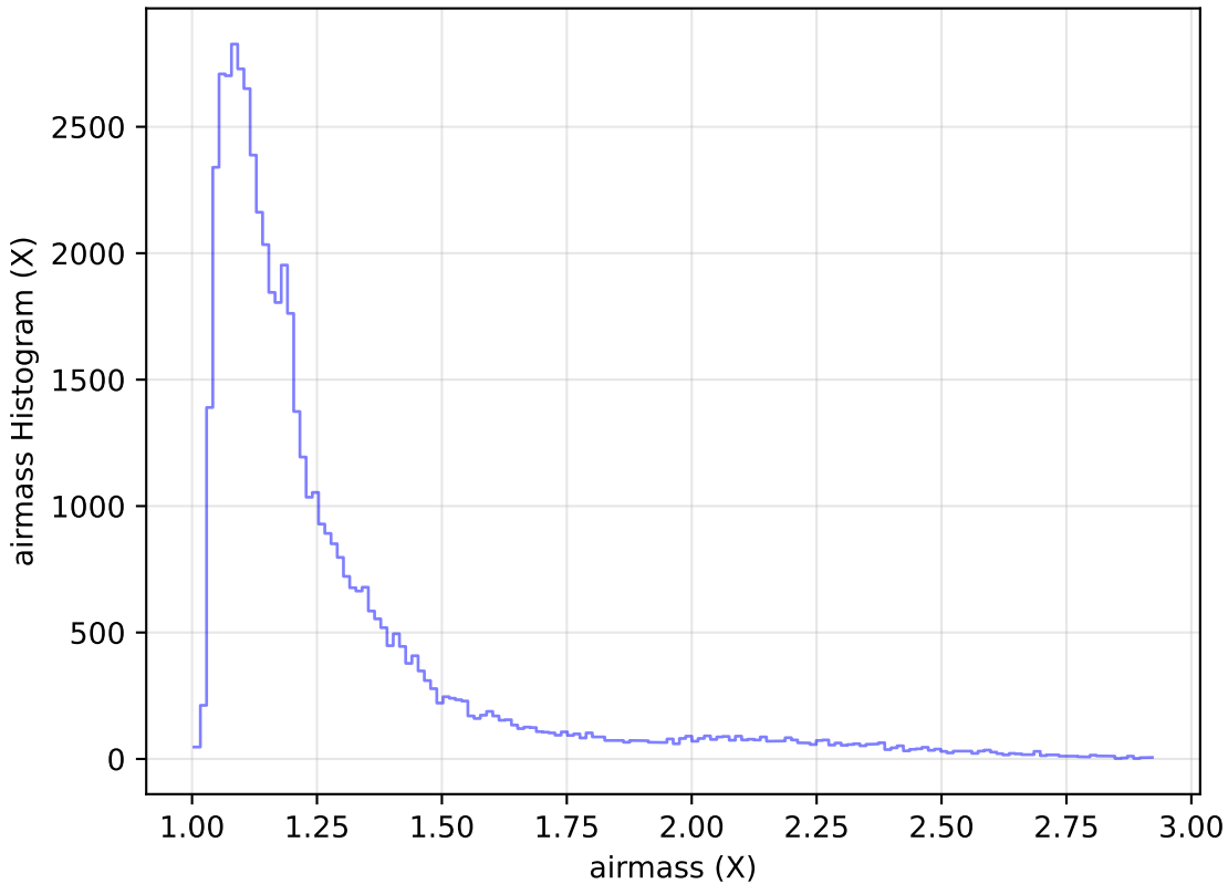
too_elab_r16_d2_ugrizy_v3.4_10yrs Yr 1 i band: airmass Histogram
