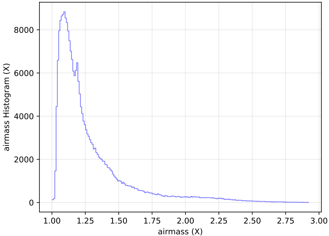
too_elab_r16_d2_ugrizy_v3.4_10yrs Yr 1 all bands: airmass Histogram
