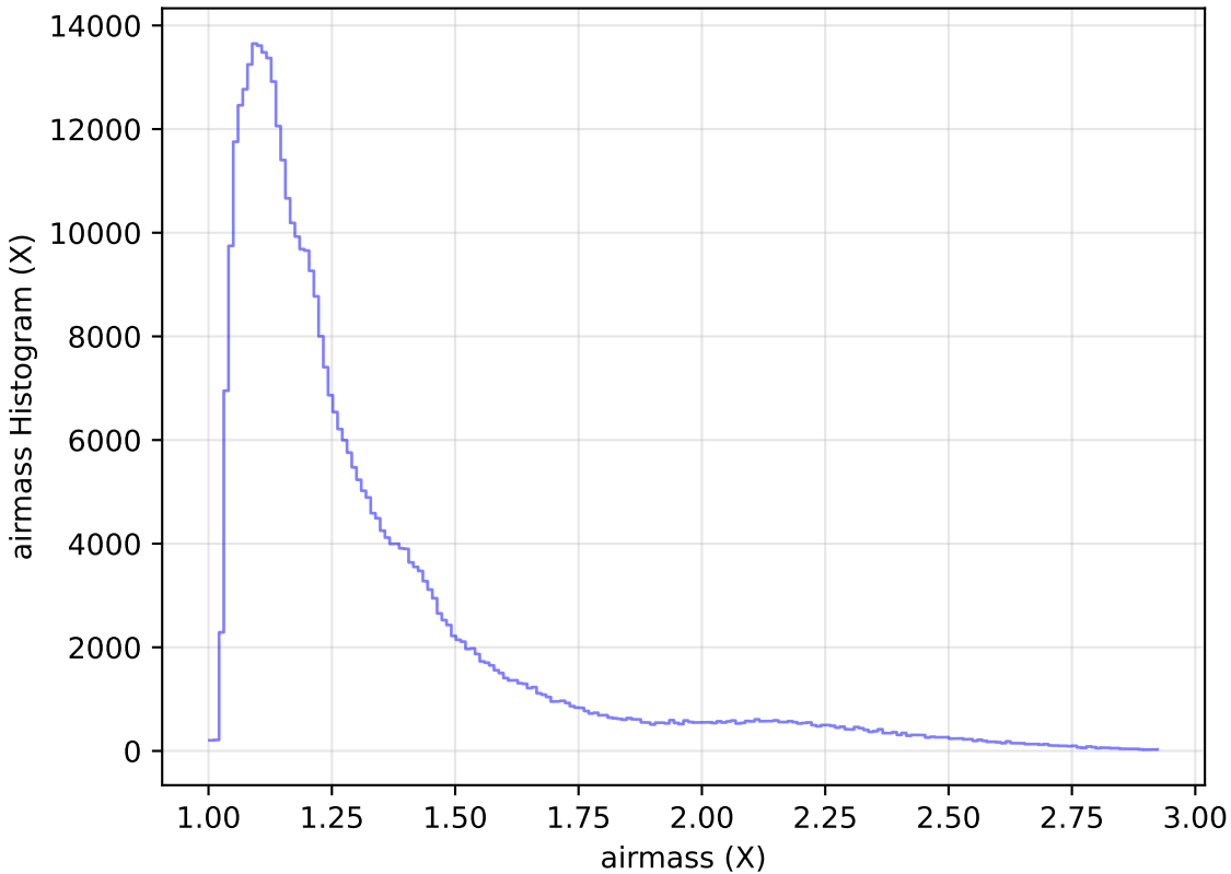
too_elab_r16_d2_ugrizy_v3.4_10yrs WFD z band: airmass Histogram
