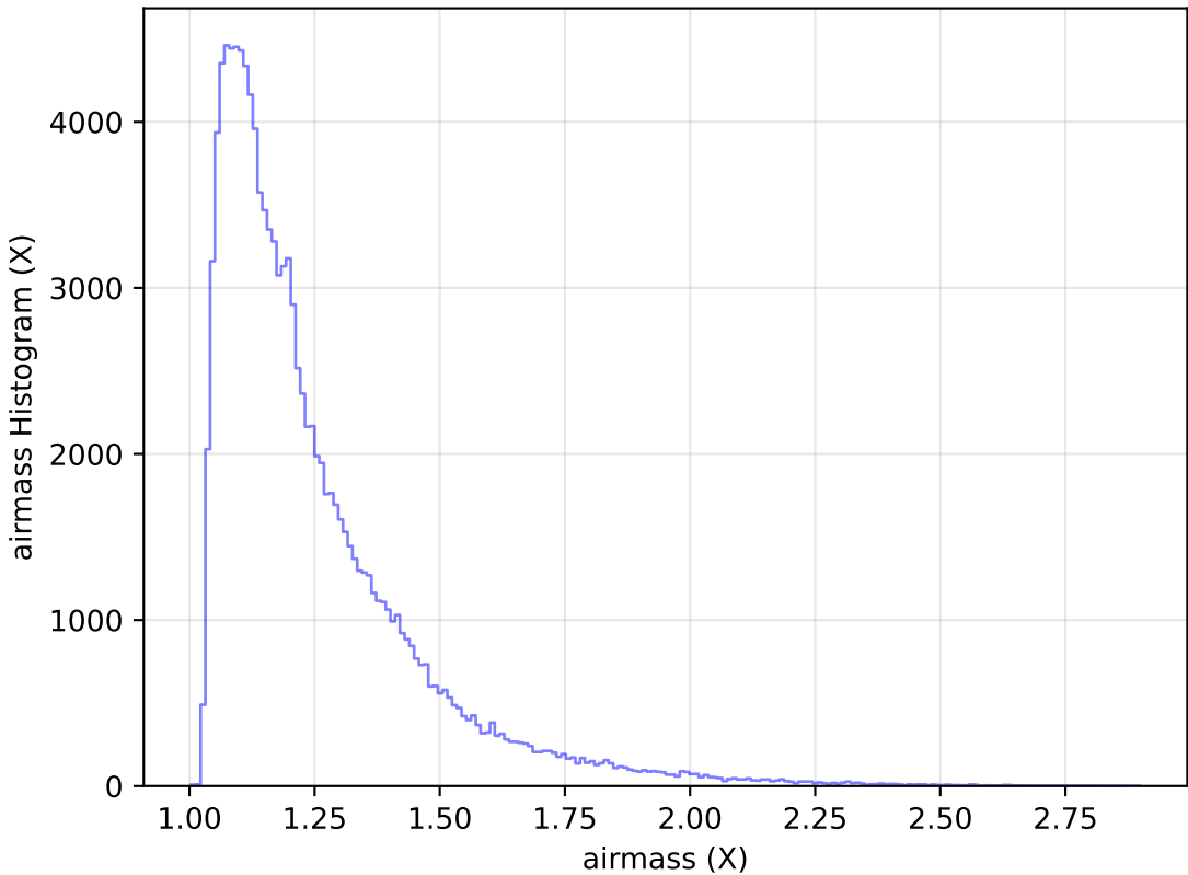
too_elab_r16_d2_ugrizy_v3.4_10yrs WFD u band: airmass Histogram
